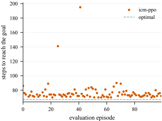
Steps to goal (eval) -- Dilution-50@4002
