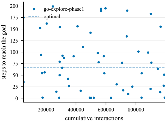
Steps to goal (train) -- Dilution-50@4002
