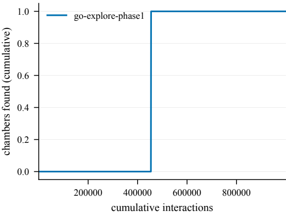
Chambers -- GiveUp1-100@4000
