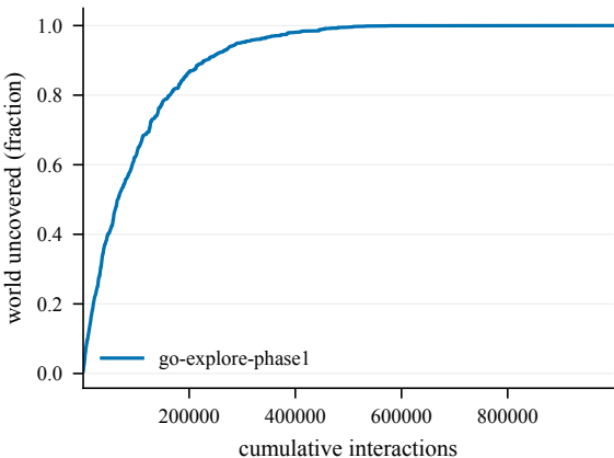
Cumulative coverage -- GiveUp1-100@4000
