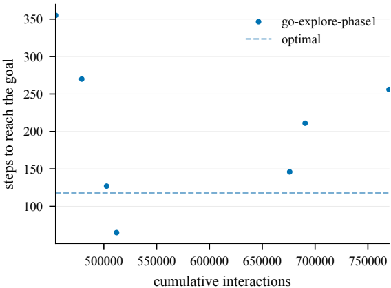
Steps to goal (train) -- GiveUp1-100@4000
