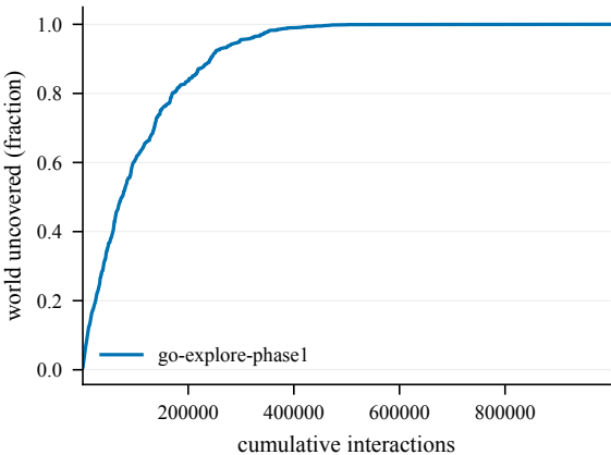
Cumulative coverage -- GiveUp1-100@4001
