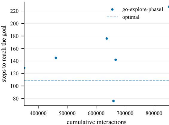
Steps to goal (train) -- GiveUp1-100@4001
