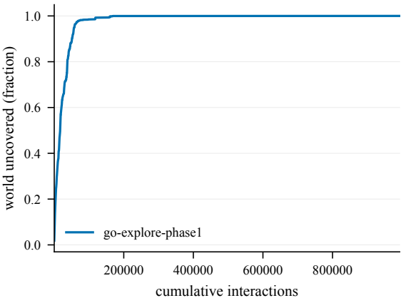
Cumulative coverage -- GiveUp1-50@4000
