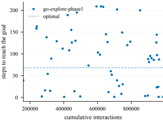
Steps to goal (train) -- GiveUp1-50@4000
