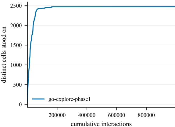
States discovered -- GiveUp1-50@4000
