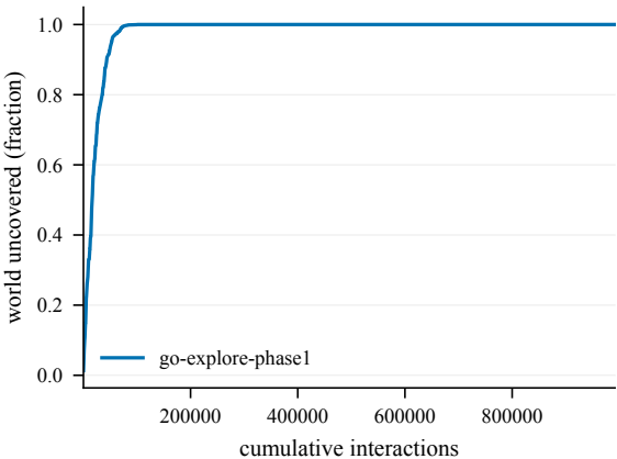
Cumulative coverage -- GiveUp1-50@4001
