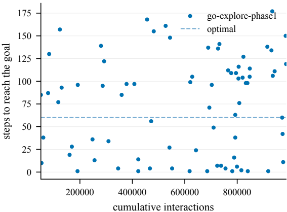
Steps to goal (train) -- GiveUp1-50@4001
