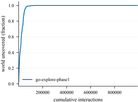
Cumulative coverage -- GiveUp1-50@4002
