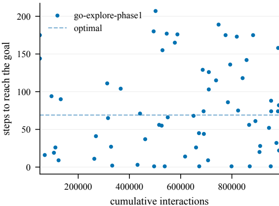
Steps to goal (train) -- GiveUp1-50@4002
