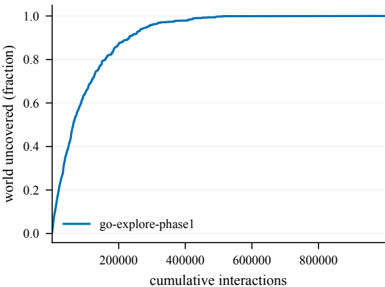
Cumulative coverage -- GiveUp2-100@4000
