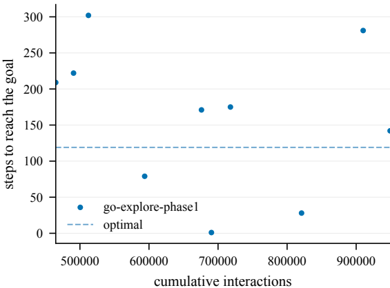
Steps to goal (train) -- GiveUp2-100@4000
