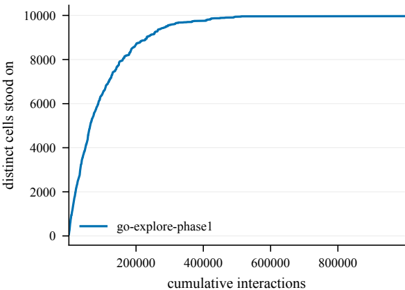
States discovered -- GiveUp2-100@4000
