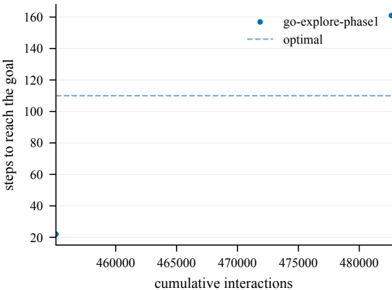
Steps to goal (train) -- GiveUp2-100@4001
