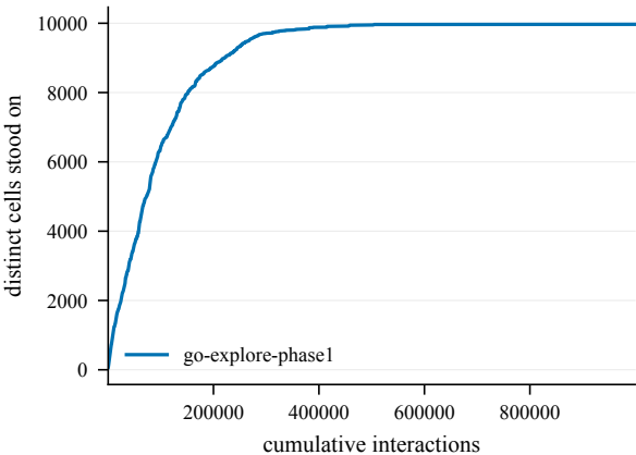
States discovered -- GiveUp2-100@4001
