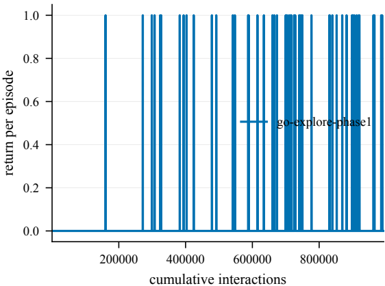
Return -- GiveUp2-50@4000
