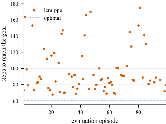
Steps to goal (eval) -- GiveUp2-50@4001
