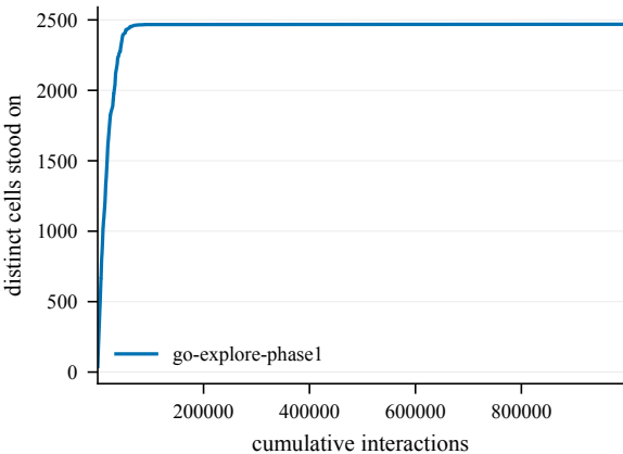
States discovered -- GiveUp2-50@4001
