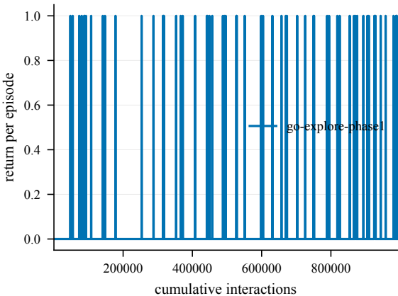
Return -- GiveUp2-50@4002
