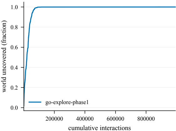
Cumulative coverage -- GiveUp2-50@4002
