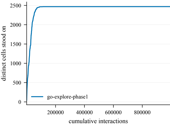
States discovered -- GiveUp2-50@4002
