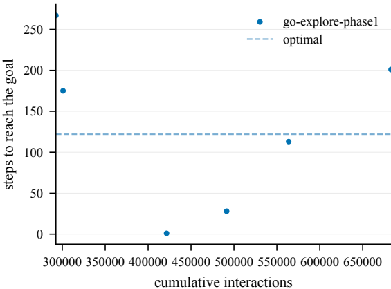
Steps to goal (train) -- GiveUp4-100@4000
