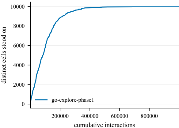
States discovered -- GiveUp4-100@4000
