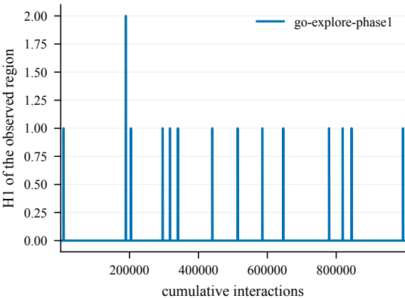
Discovered topology -- GiveUp4-100@4001
