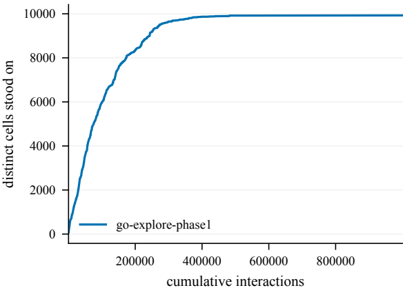
States discovered -- GiveUp4-100@4001
