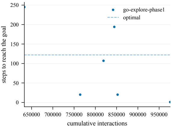
Steps to goal (train) -- GiveUp4-100@4002
