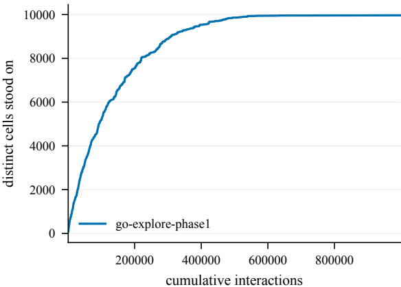
States discovered -- GiveUp4-100@4002
