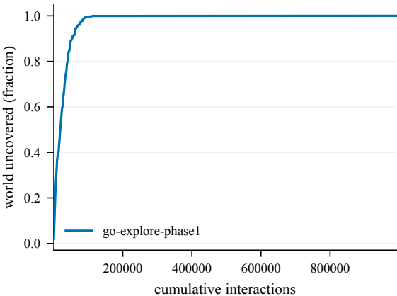
Cumulative coverage -- GiveUp4-50@4000
