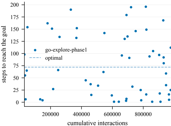
Steps to goal (train) -- GiveUp4-50@4000
