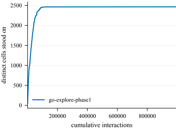
States discovered -- GiveUp4-50@4000
