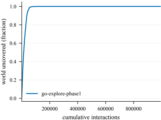
Cumulative coverage -- GiveUp4-50@4001
