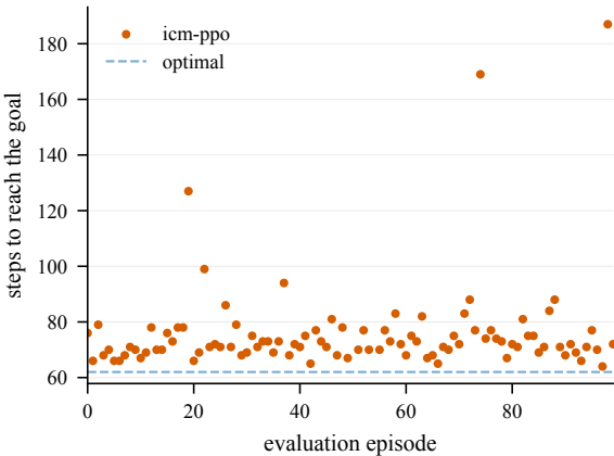
Steps to goal (eval) -- GiveUp4-50@4001
