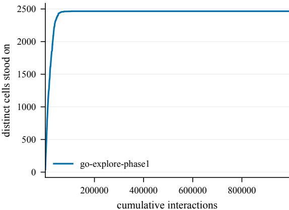
States discovered -- GiveUp4-50@4001
