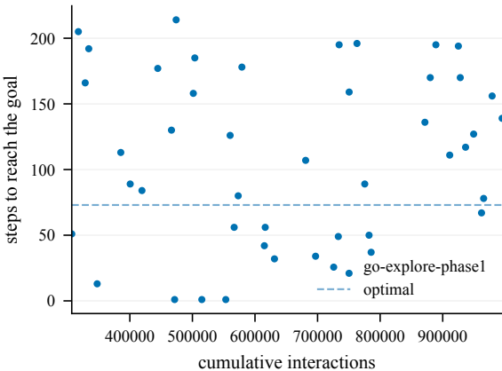
Steps to goal (train) -- GiveUp4-50@4002
