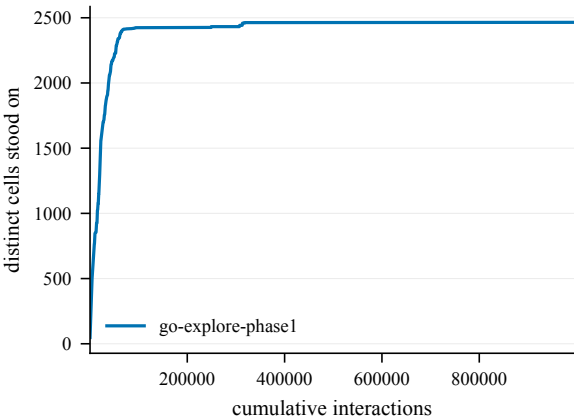
States discovered -- GiveUp4-50@4002
