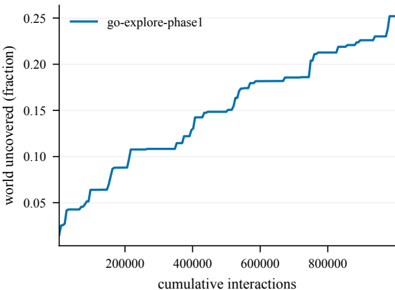
Cumulative coverage -- Maze-100@4000
