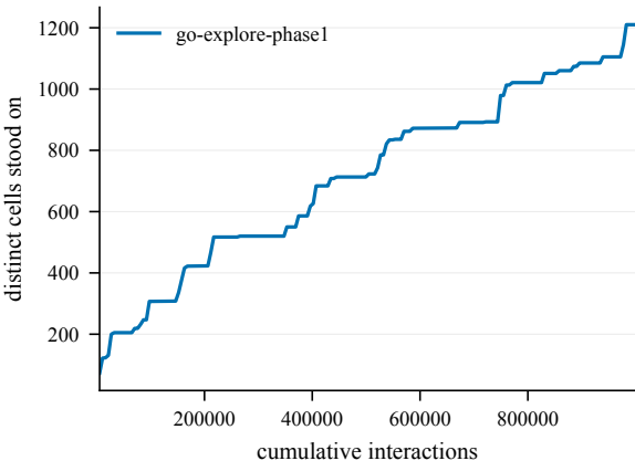
States discovered -- Maze-100@4000
