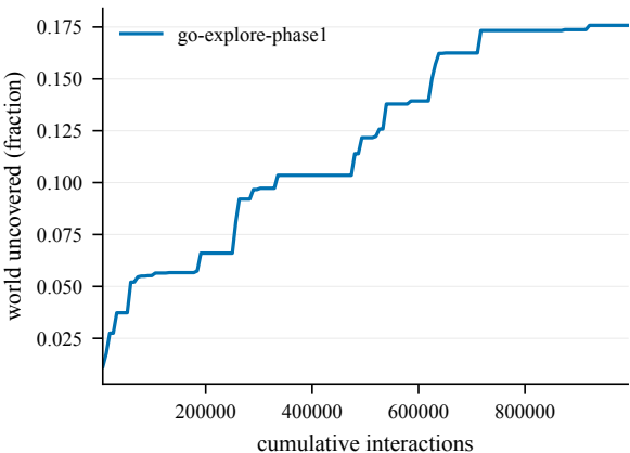
Cumulative coverage -- Maze-100@4001
