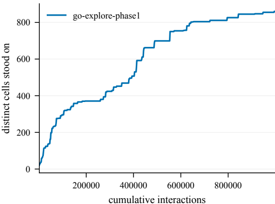
States discovered -- Maze-50@4000
