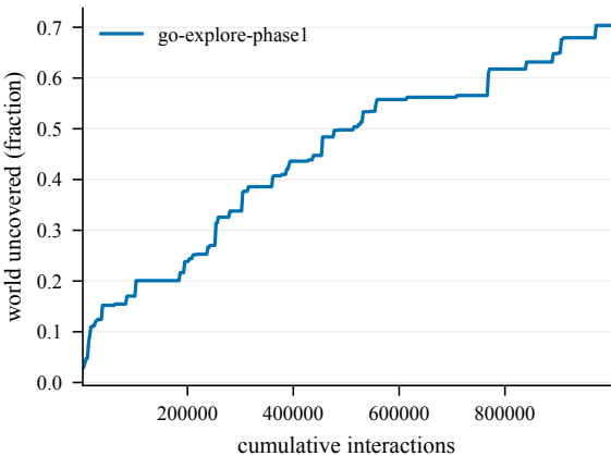
Cumulative coverage -- Maze-50@4001
