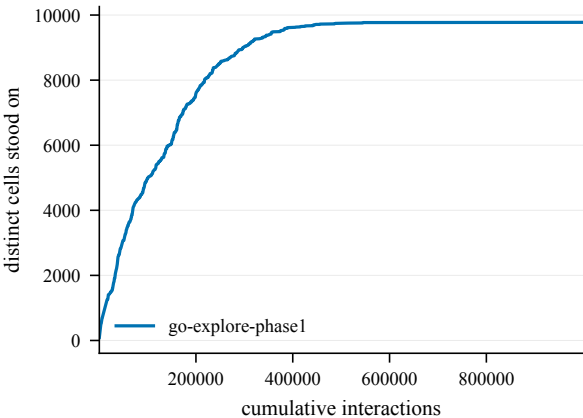
States discovered -- Nested1-100@4000
