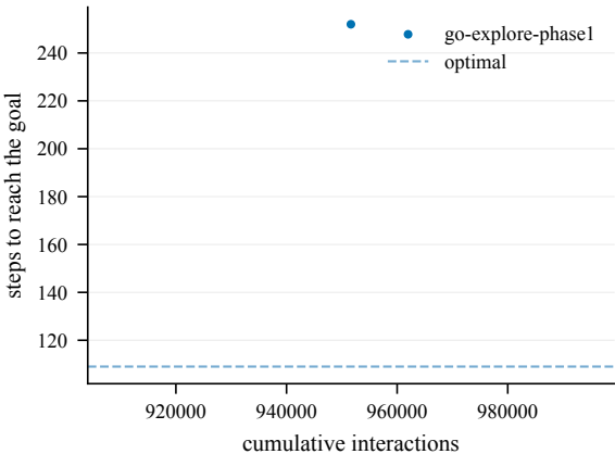
Steps to goal (train) -- Nested1-100@4001
