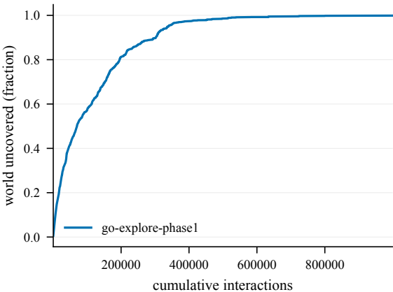
Cumulative coverage -- Nested1-100@4002
