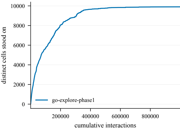
States discovered -- Nested1-100@4002
