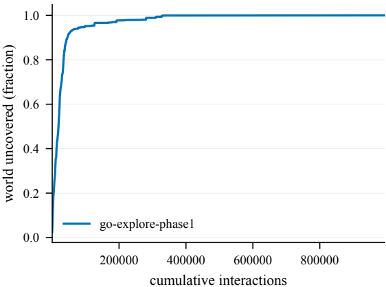
Cumulative coverage -- Nested1-50@4000
