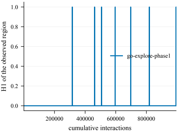
Discovered topology -- Nested1-50@4000
